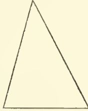
A TRIANGLE HAVING ALL ITS ANGLES ACUTE AND ITS THREE SIDES UNEQUAL.
